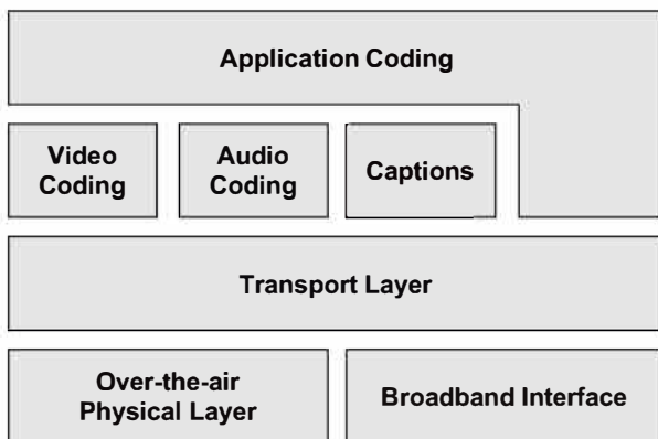
Fig. 2. TV 3.0 Architecture [2].
